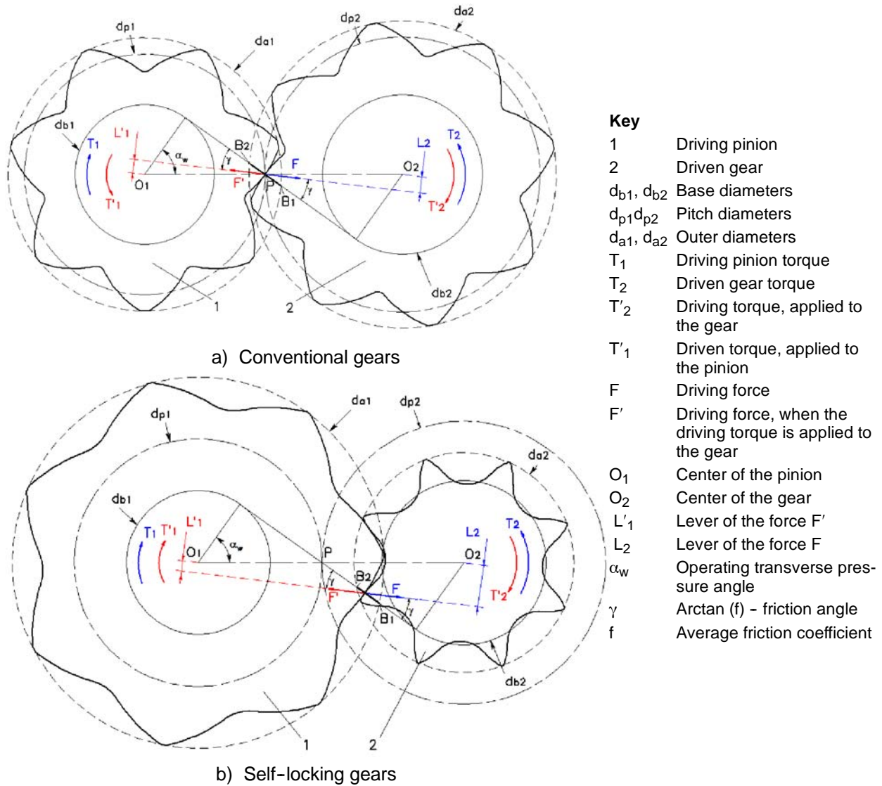
Figure 1. Conventional (a) and self-locking (b) gears driven by output load
