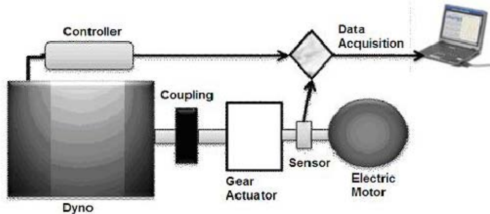
Figure 6. Helical self-locking gear actuator test bench
