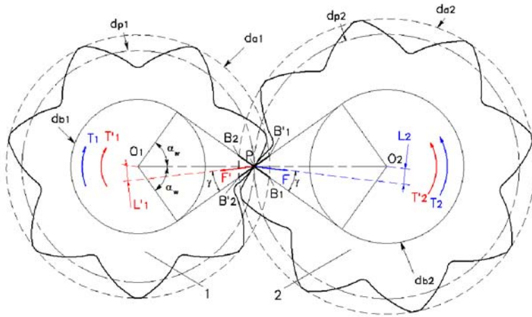
a) Conventional gears
