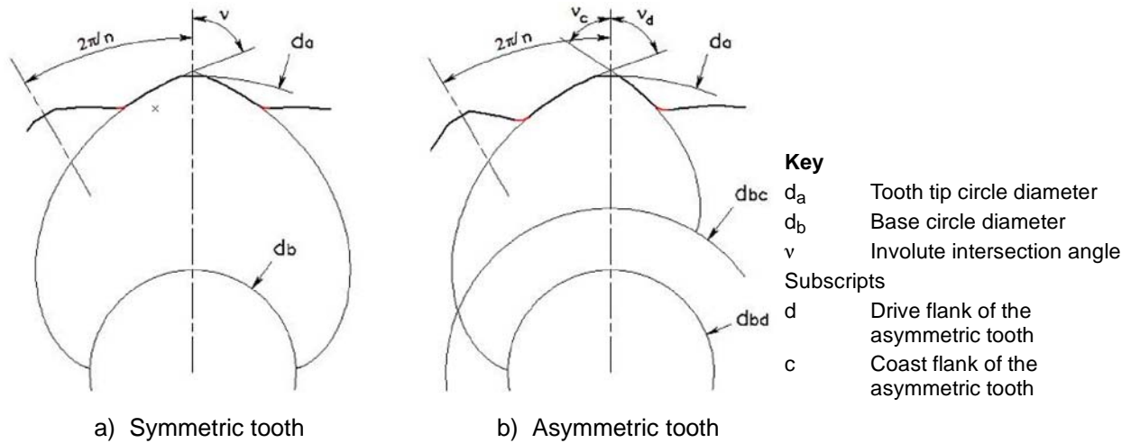
Figure 3. Direct Gear Design® tooth profile definition;
